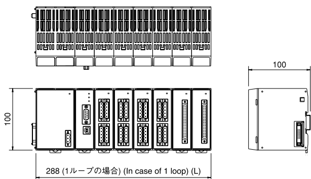
制御装置寸法図 (DINレール取付け時の外形寸法です。) Control device dimensional drawing (outside dimension when DIN rail is mounted).
